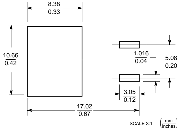
VIEW W-W 3
